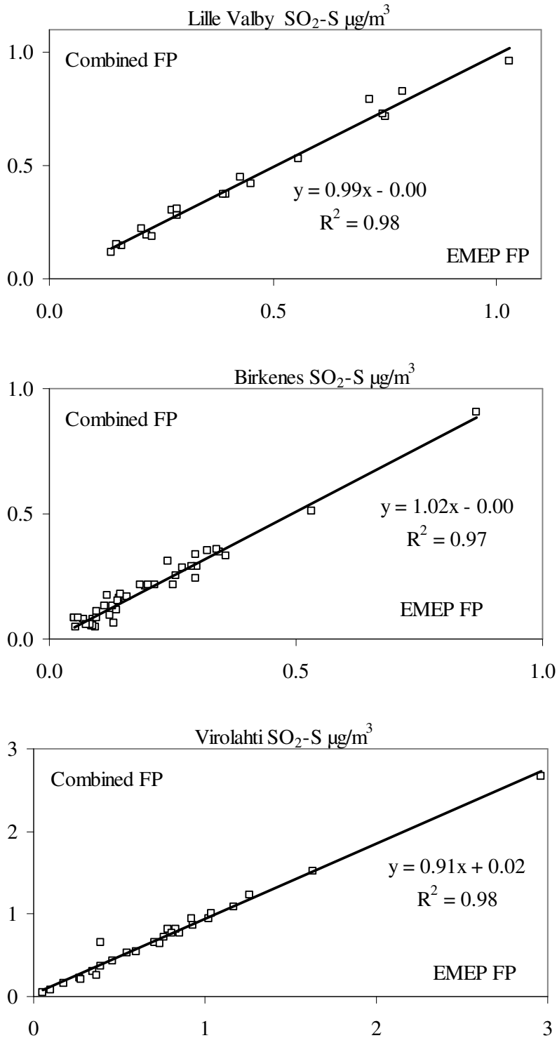
Fig. 8. The sulphur dioxide concentration collected with the combined filter pack as a function of the sulphur dioxide concentration collected with the EMEP filter pack.
