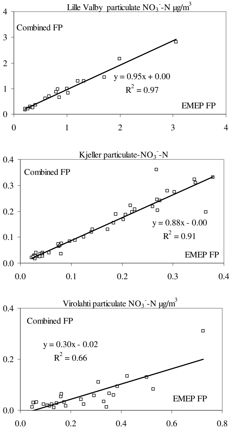
Fig. 5. The particulate nitrate concentration collected with the combined filter pack as a function of the particulate nitrate concentration collected with the EMEP filter pack.
